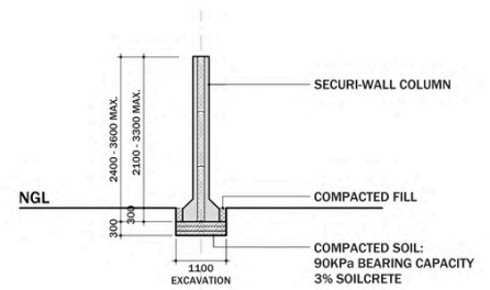
TYPICAL SECTION - BOUNDARY WALLING
