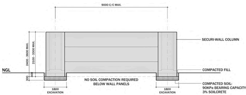
TYPICAL ELEVATION - BOUNDARY WALLING
